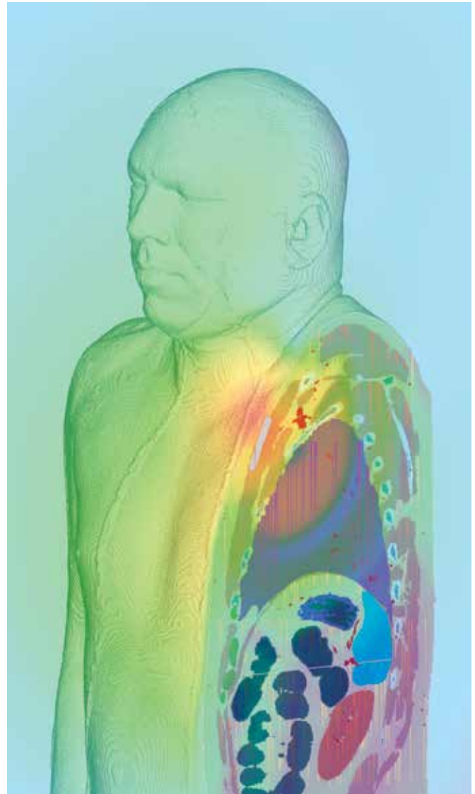
Life Sciences: Electric field from a pacemaker antenna inside the human body.
